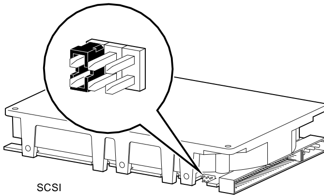
Figure 1 SCSI ID for the RZ25L Fixed Disk Drive
