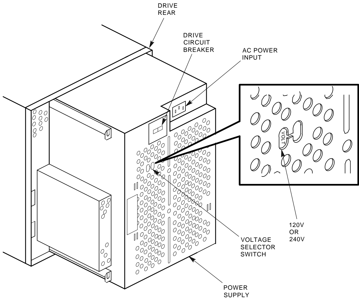
Figure 3-4 RA90/RA92 Voltage Selector Switch/Circuit Breaker
