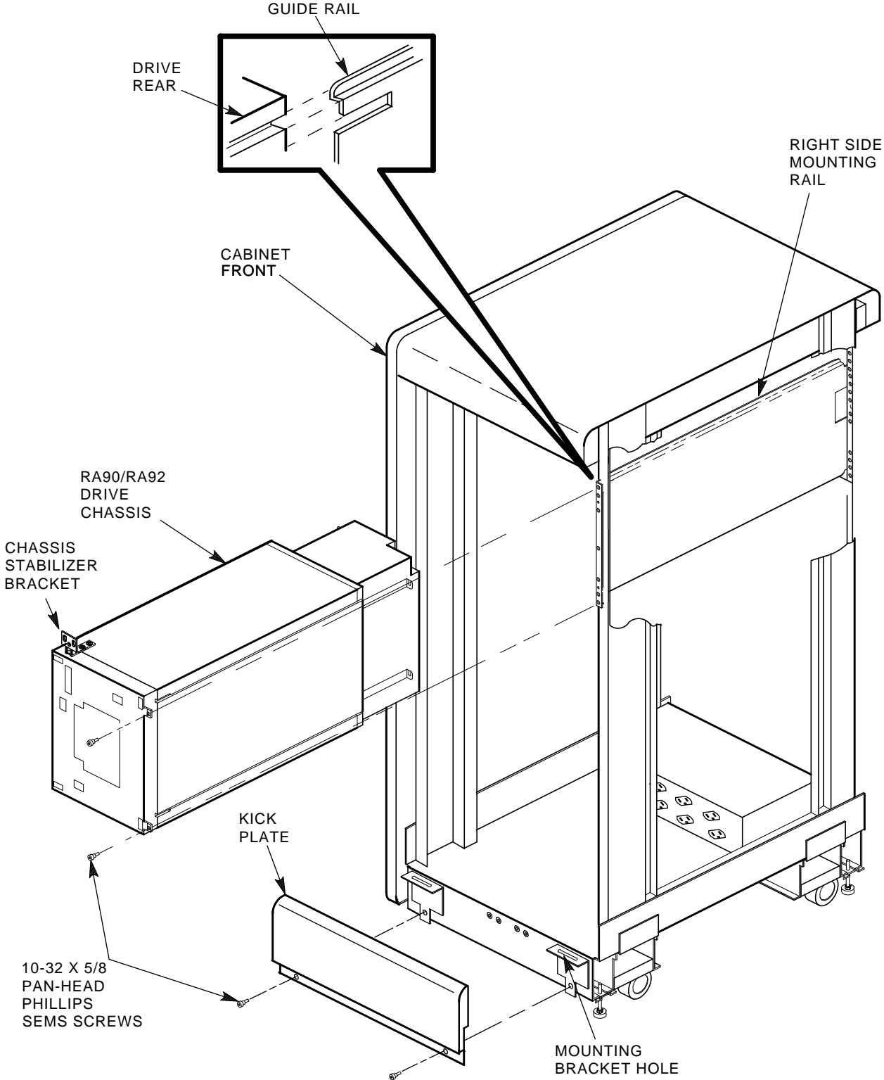
Figure 2-4 Cabinet Rails and Kick Plate (Front)
