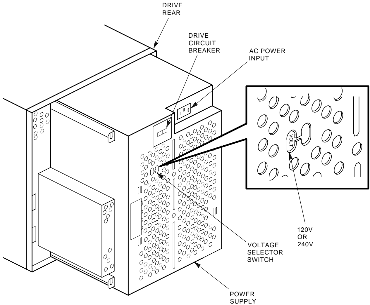
Figure 2-7 RA90/RA92 Voltage Selector Switch/Circuit Breaker
