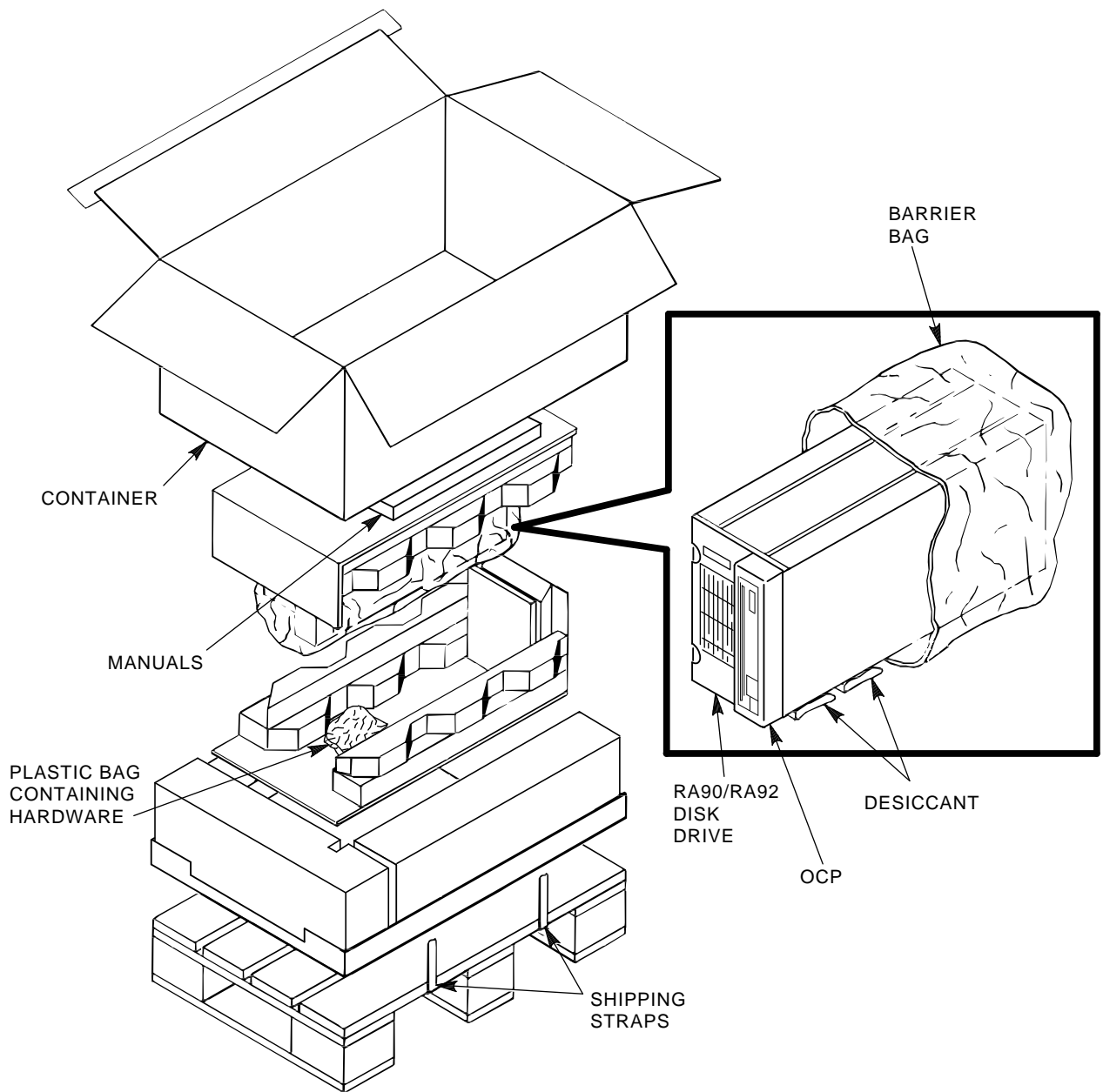
Figure 1-2 RA90-NA/RA92-NA Add-On Shipping Container Contents
