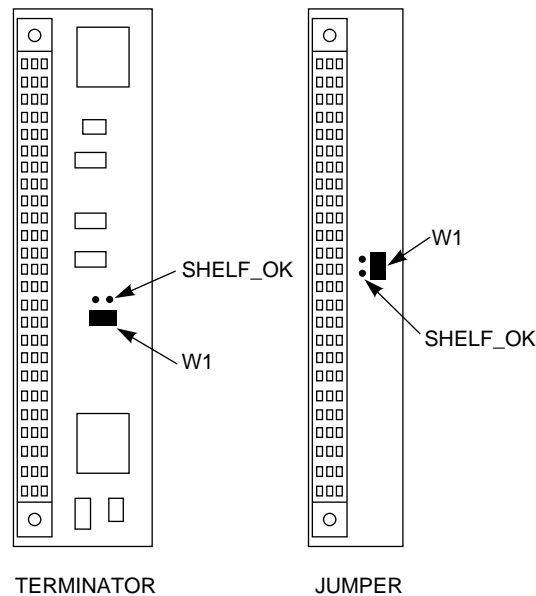
Figure 2-2 SHELF_OK Disabled
