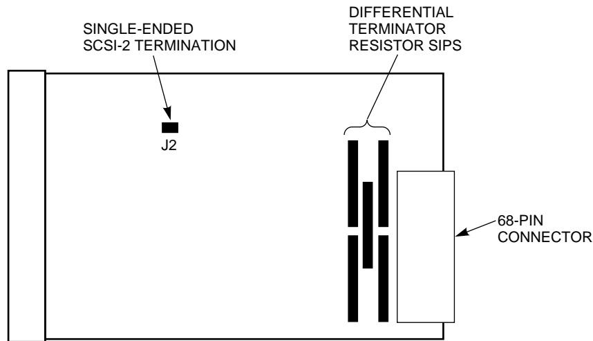
Figure 6-2 End-Bus DWZZA Bus Terminators
