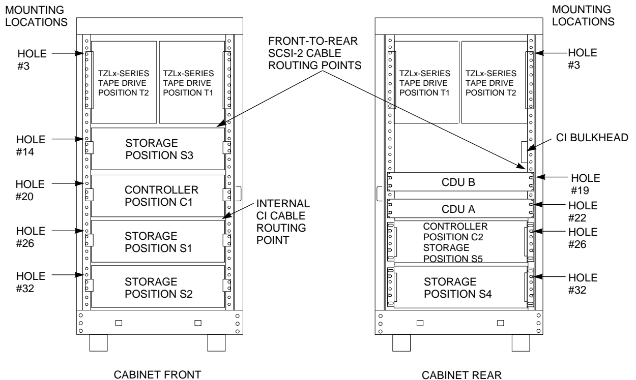
Figure 5–2 SH043 Controller/Storage Cabinet Shelf and Tape Drive Locations
