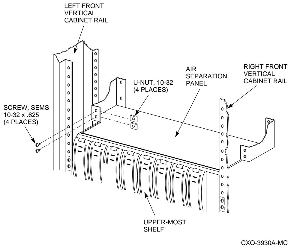
Figure 6–4 Front Air Separation Panel Installation
