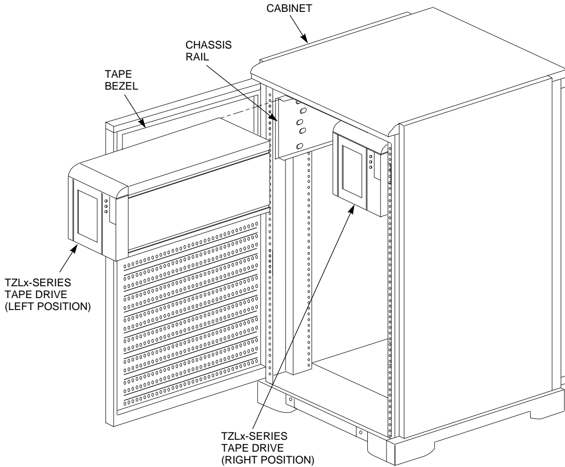
Figure 7-1 TZLX-Series Tape Drive Installation
