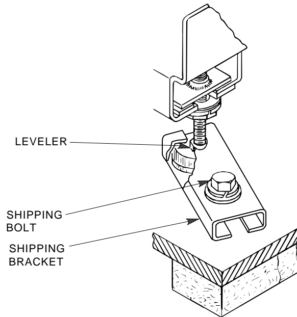
Figure 3–3 Shipping Bolts and Brackets
