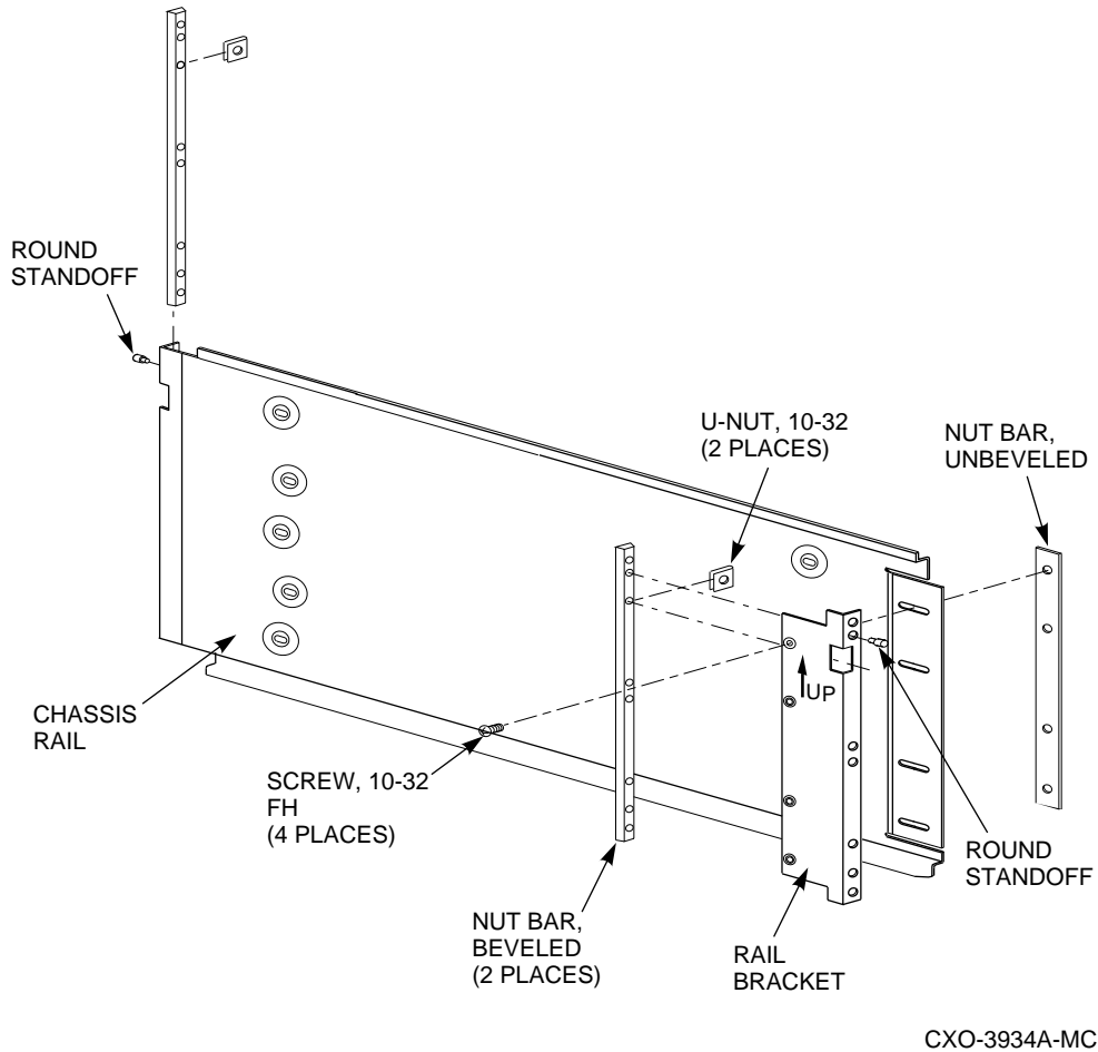
Figure 7-3 Chassis Rail Assembly
