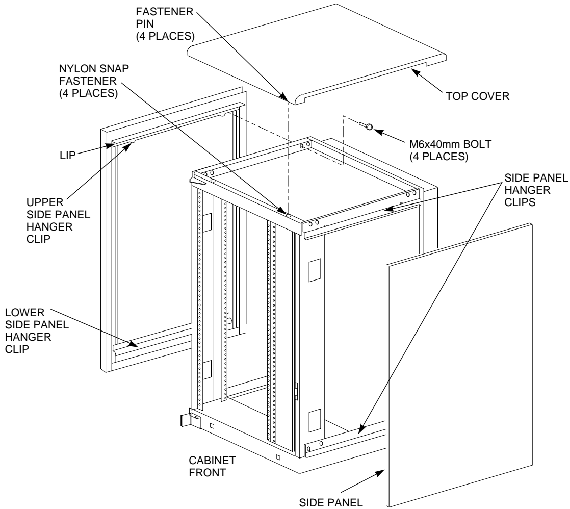
Figure 6–1 Exterior Cabinet Panel Removal and Installation
