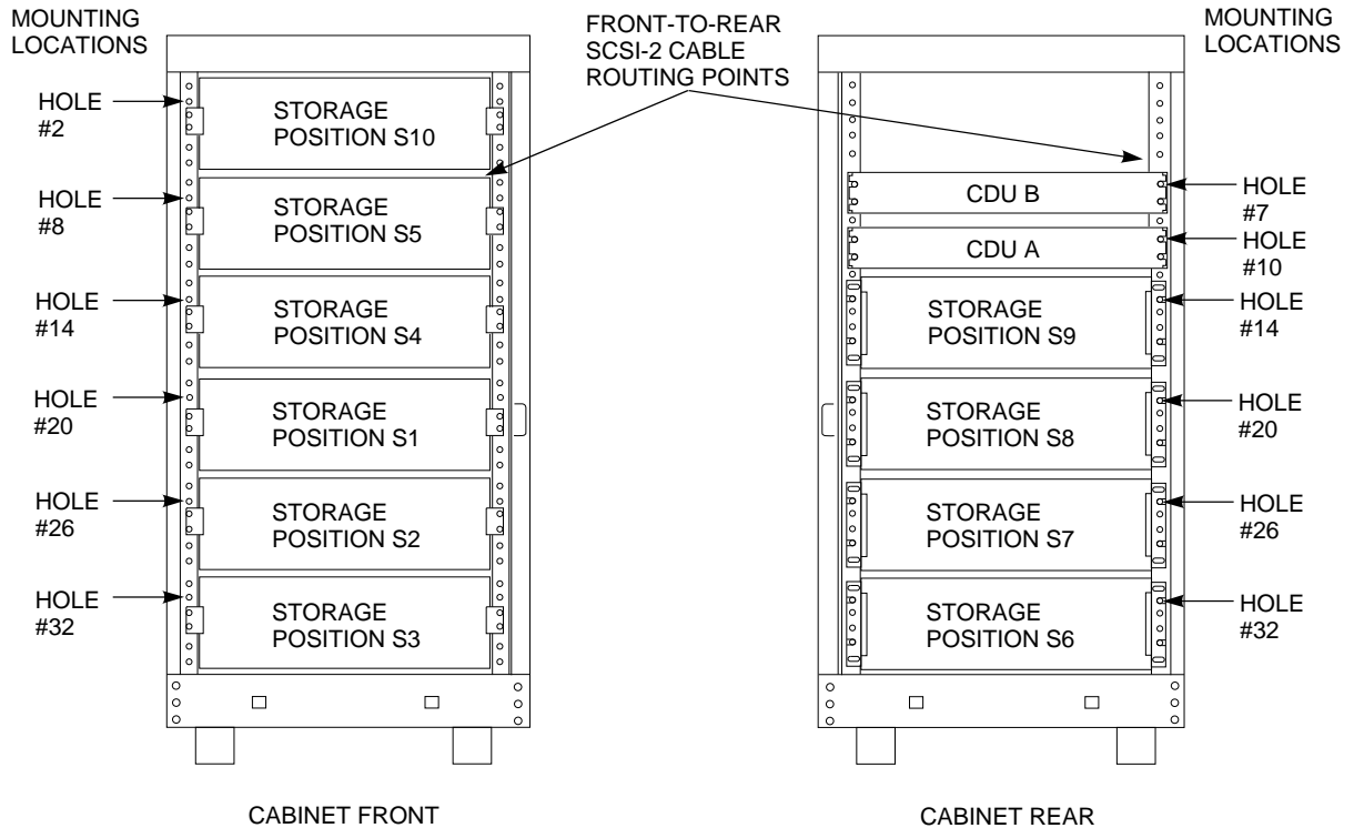
Figure 4–1 SH043 Storage-only Cabinet Shelf Locations
