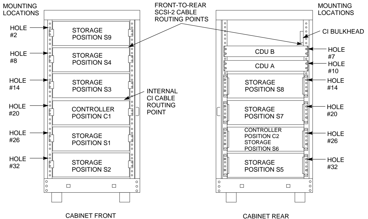
Figure 5-1 SH043 Controller/Storage Cabinet Shelf Locations
