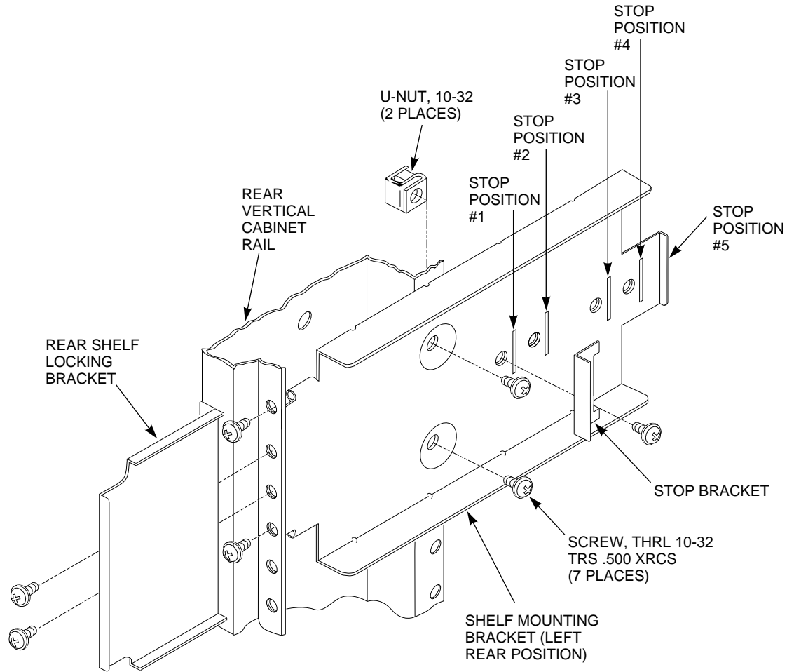
Figure 6–3 Rear Shelf Bracket Installation
