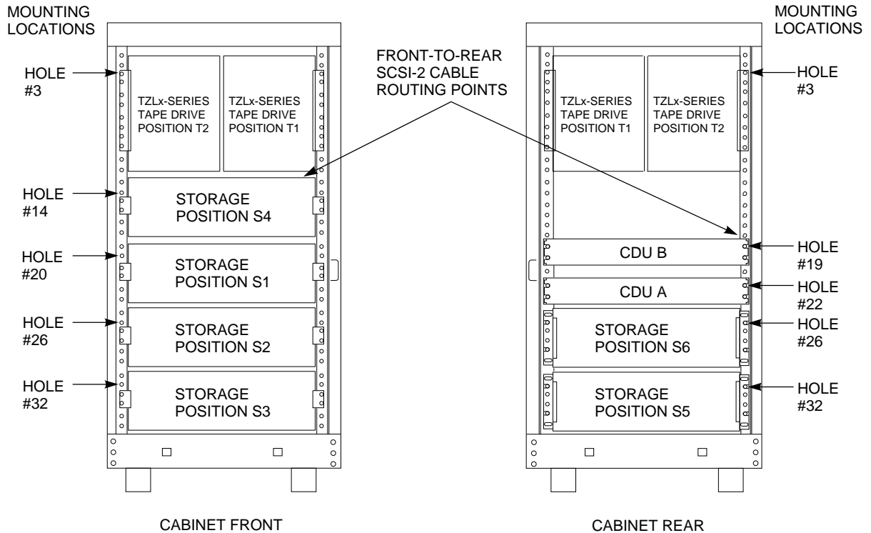
Figure 4–2 SH043 Storage-only Cabinet Shelf and Tape Drive Locations
