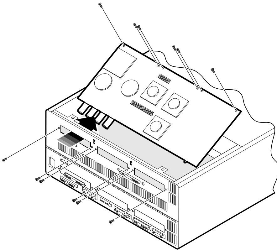
Figure 2-5 Module Removal
